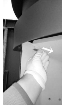
3. Pull out the deflector pin. Both sides evenly.
